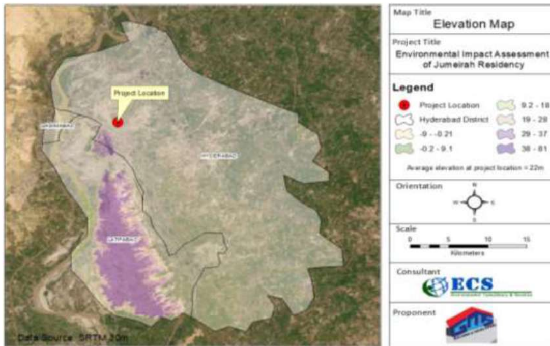
Figure 2: Land Elevation Map of Project Site
