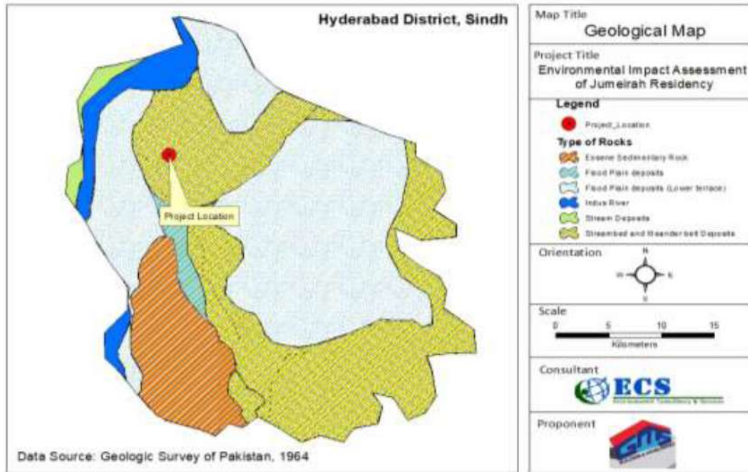
Figure 3: Geological Map
