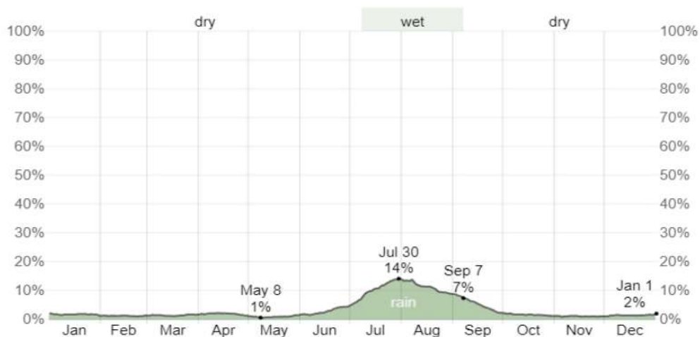
Figure 7: Precipitation Trend in Hyderabad
