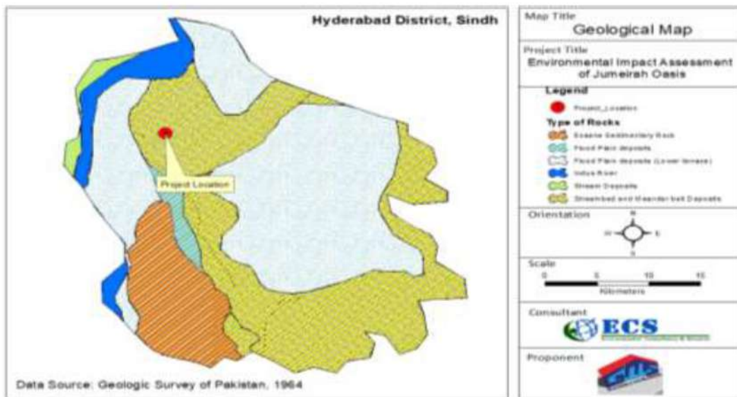
Figure 3: Geological Map
