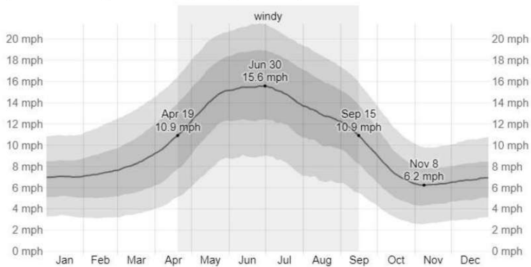
Figure 6: Wind speed experienced in Hyderabad
