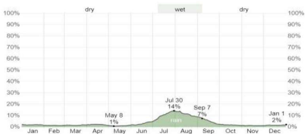
Figure 7: Precipitation Trend in Hyderabad
