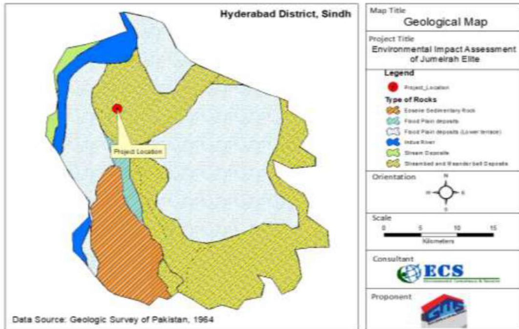
Figure 3: Geological Map
